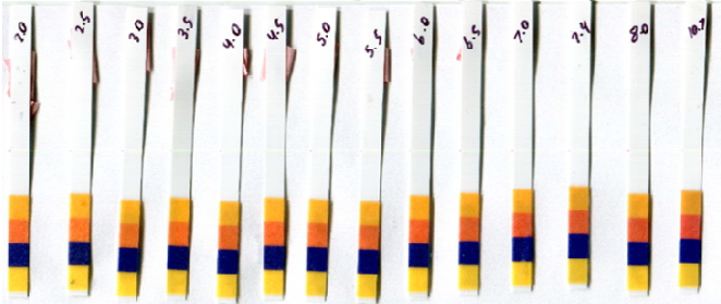
Supplemental Figure 1 | pH of reaction solution before and after quenching with 0.1 M Gly-NaOH pH 10.7
