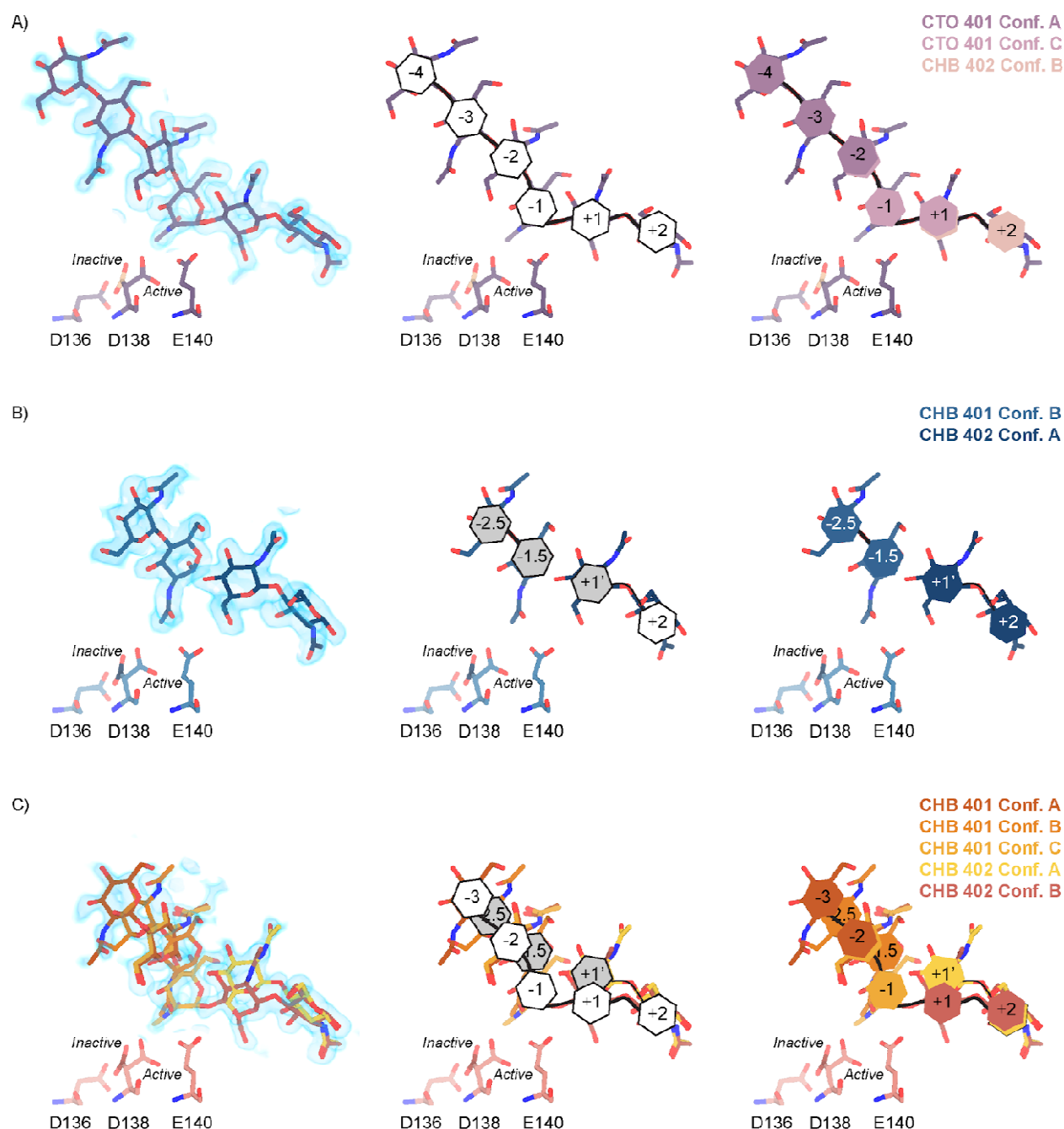
Figure 2 | Schematic representation of sugar-binding subsites in mAMCase.
