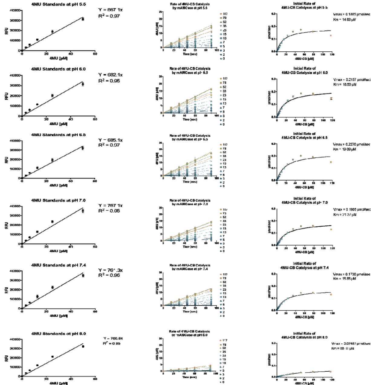
Supplemental Figure 2 | Kinetics of 4MU-chitobioside catalysis by mAMCase catalytic domain at various pH.
