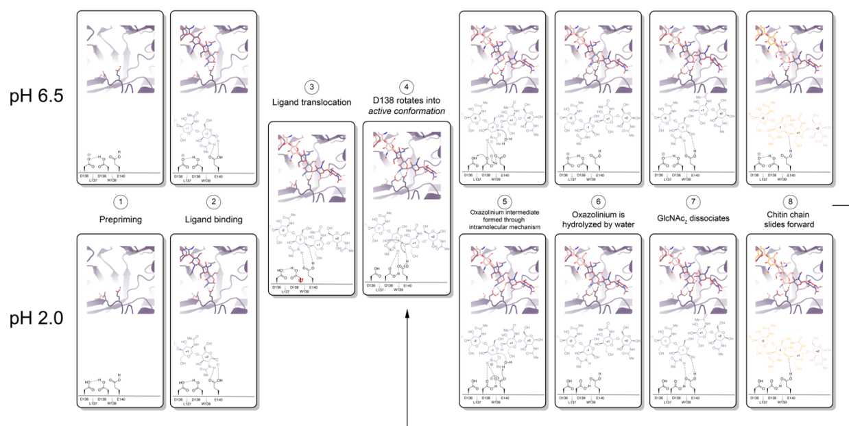
Figure 6 | Proposed model for ligand translocation towards the active site and ligand release post-catalysis.
