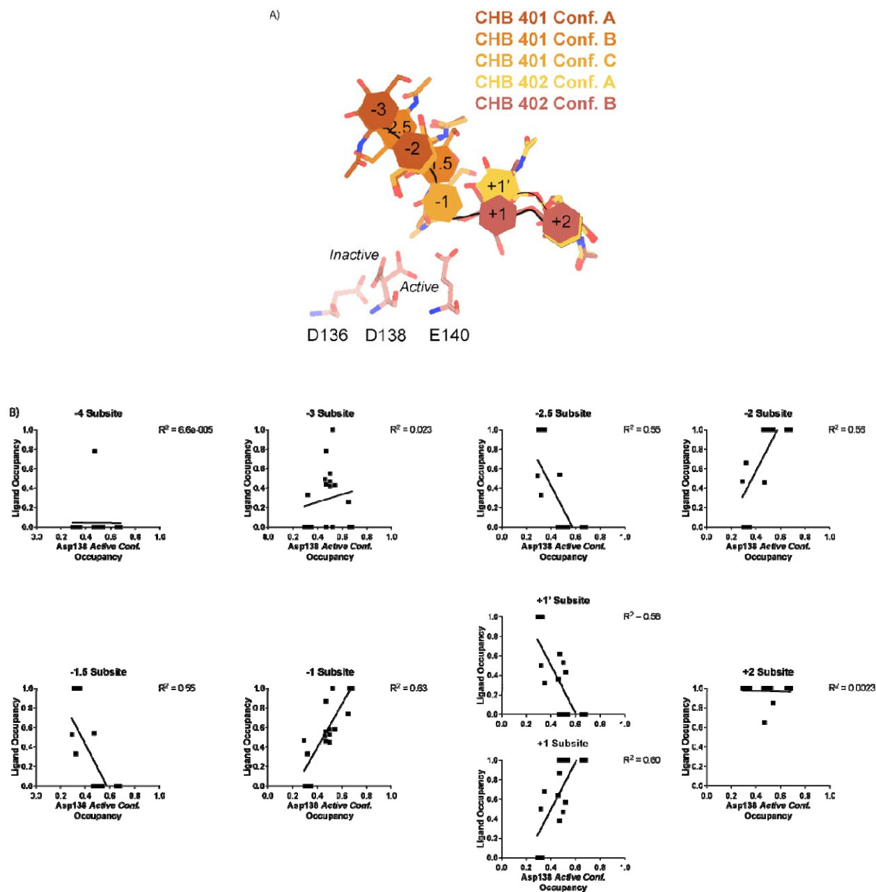
Figure 3 | Asp138 orientation correlates with ligand subsite occupancy.
