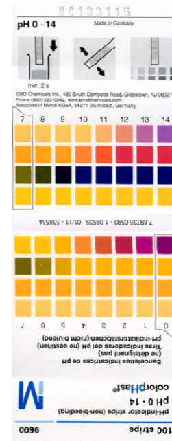
Supplemental Figure 1 | pH of reaction solution before and after quenching with 0.1 M Gly-NaOH pH 10.7
